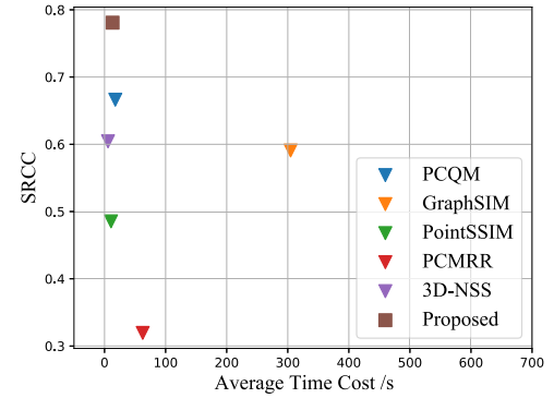
Fig. 10. Results of computational efficiency comparison. The SRCC indicates the average SRCC values of corresponding PCQA methods on the SJTU-PCQA, WPC, and LSPCQA-I databases. The average time cost represents the average running time of the PCQA methods to evaluate a single point cloud.
