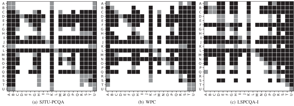
Fig. 8. Statistical test results of the proposed method and compared metrics on the SJTU-PCQA, WPC, and LSPCQA-I databases. A black/white block means the row method is statistically worse/better than the column one. A gray block means the row method and the column method are statistically indistinguishable. The metrics are denoted by the same index as in Table I.
