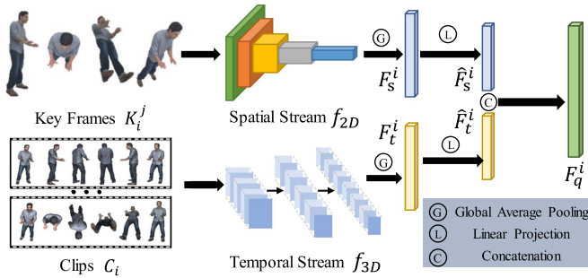
Fig. 6. Detailed structure of the feature extraction.
