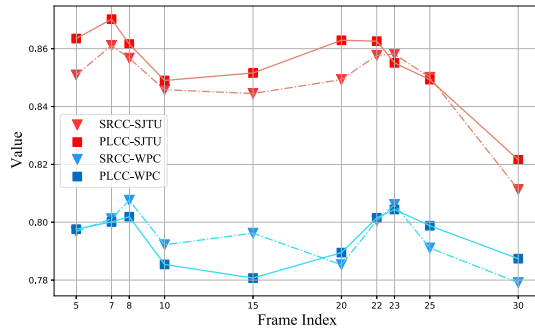
Fig. 9. Performance comparison of different key frame selection on the SJTU-PCQA and WPC databases. The 7-th frame is the proposed key frame selection.
