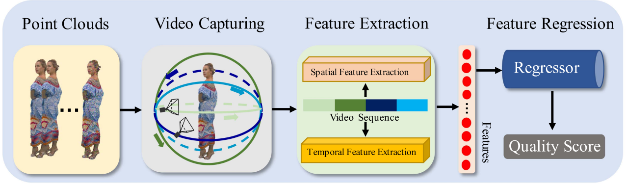
Fig. 3. Framework of the proposed method, which includes the video capture process, the feature extraction module, and the feature regression module.
